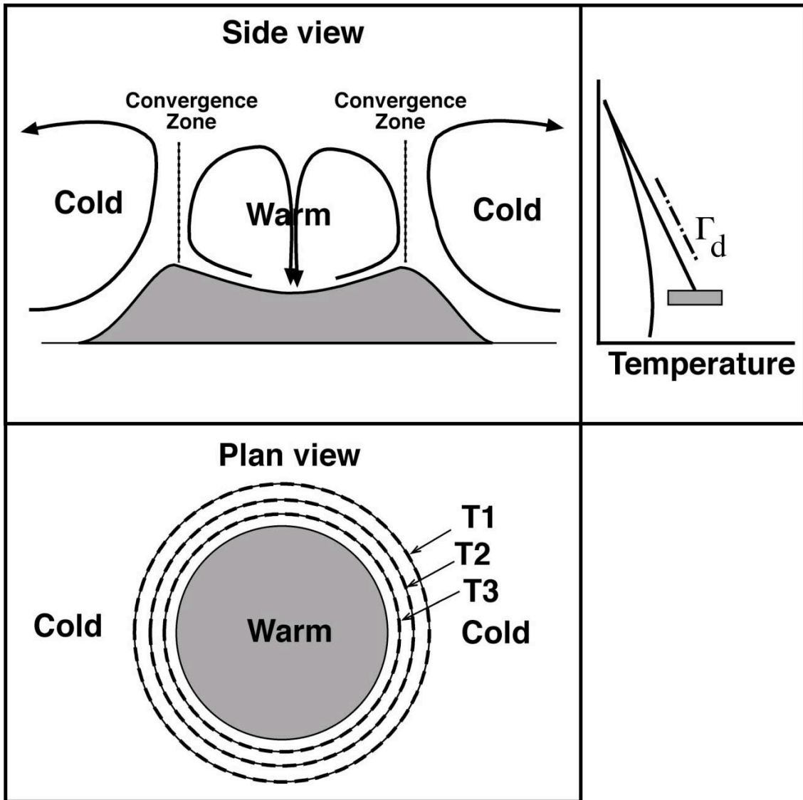
Figure 14. Schematic diagram of daytime circulations and temperature profiles above and alongside an elevated circular plateau, illustrating the daytime buildup of a baroclinic zone at the edges of the plateau that leads to a break-in of cold winds onto the plateau in the evening. The dry adiabatic lapse rate \Gamma_d is provided as a reference.
