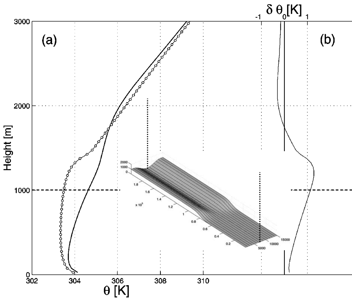
Figure 9. (a) Comparison of different vertical profiles of potential temperature in an idealized valley-plain system (sketched in the insert). The profiles are taken along the valley axis (solid line) and over the plain (line of circles) along the dashed vertical lines indicated in the insert at t = 6 h after simulated sunrise. (b) Difference between the two profiles at various heights. The horizontal dashed line at 1000 m indicates the sidewall ridge height. (Adapted from Rampanelli et al. 2004. © American Meteorological Society. Reprinted with permission).
