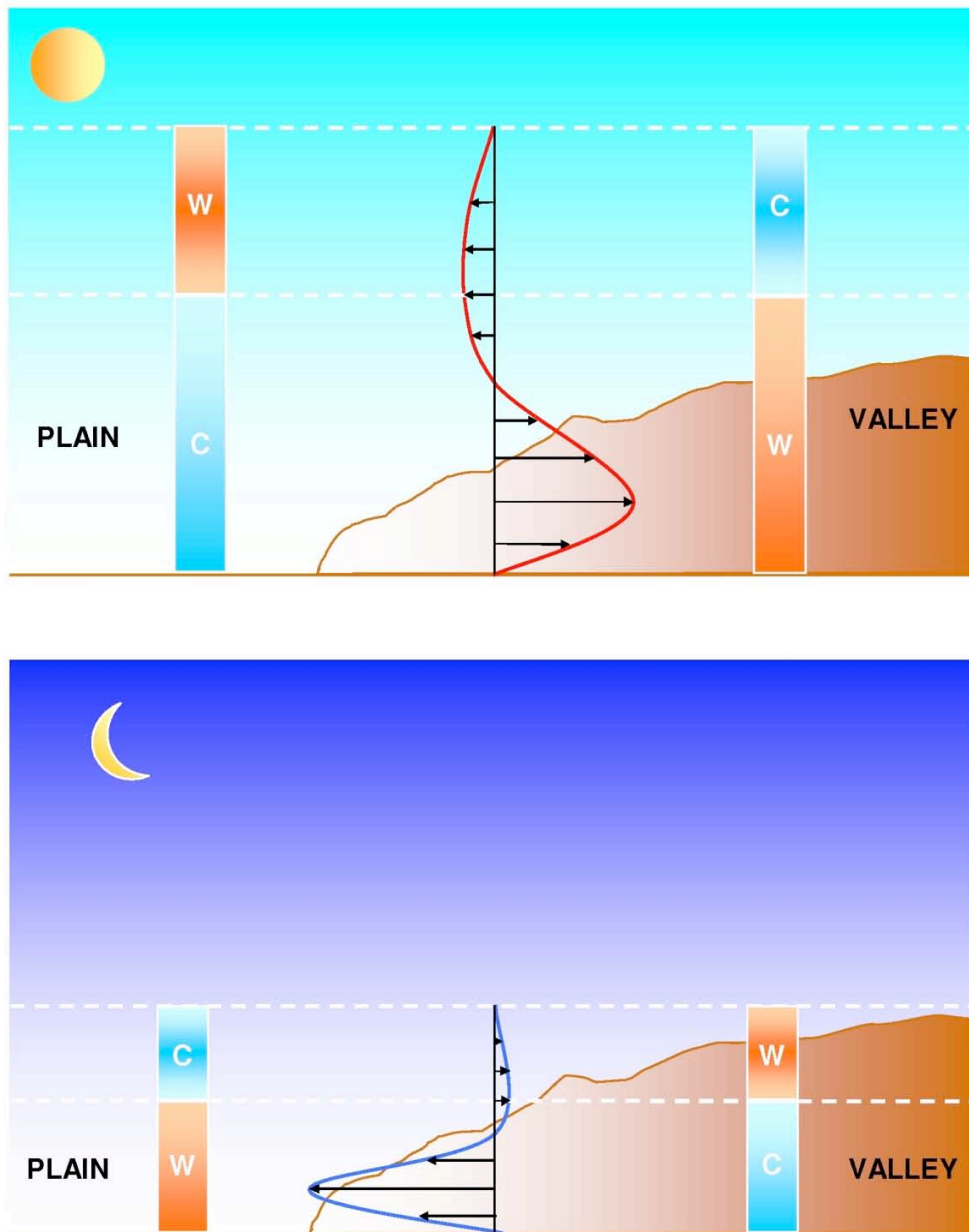
Figure 8. Idealized picture of the development of daytime up-valley winds (upper panel) and nighttime down-valley winds (lower panel) in a valley-plain system with a horizontal floor. The red and blue curves are vertical profiles of the horizontal valley wind component at a location close to the valley inlet. Two columns of air are shown – one over the valley floor and one above the plain. Red and blue sections of the columns indicate layers where potential temperature is relatively warm (W) or cold (C). The free atmosphere is assumed to be unperturbed by the daily cycle at the tops of the columns. Adapted from Whiteman (2000).
