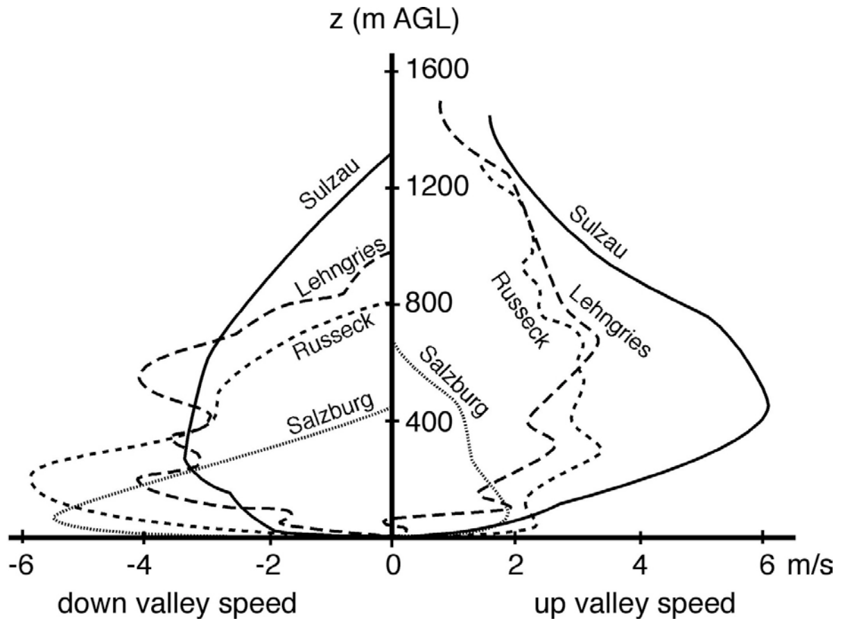
Figure 10. Average up- and down-valley wind profiles from four valleys using all daytime and nighttime data from the locations indicated (Ekhart 1944), © E. Schweizerbart Science Publishers ( www.borntraeger.cramer.de ). Used with permission.
